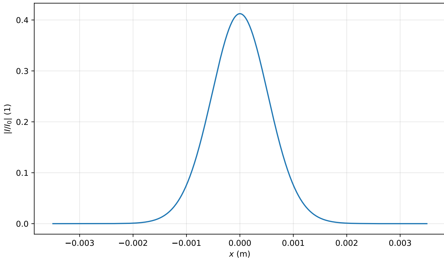
Intensity profile I(x, y = 0, z = 2.786m)/I_0 , P_{in}=0.2P_{cr} , artificial time
